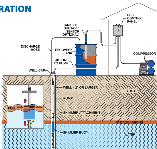
Typical PRS Installation with Optional Tankfull Shut-Off Sensor
