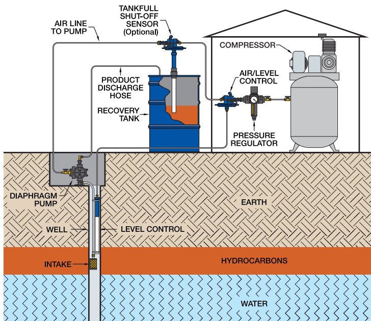
Standard Geotech TFS Configuration
